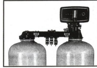
Packaged Vision™ NutriFilter™ with twin tank accessories: 3- Sample Valves
